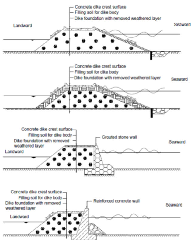
Figure 2: Different types of sea dike cross sections in the coastal reservoir
