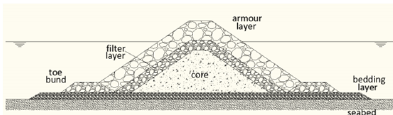
Figure 1: Typical features of sea dike
