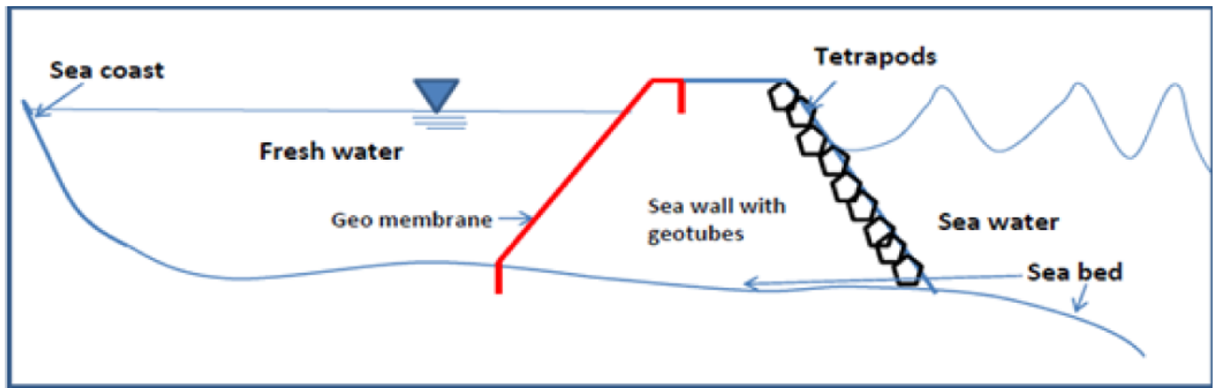
Figure 3: A typical impermeable sea dike for the coastal reservoir, Thallak G Sitharam, 2016 [3]
