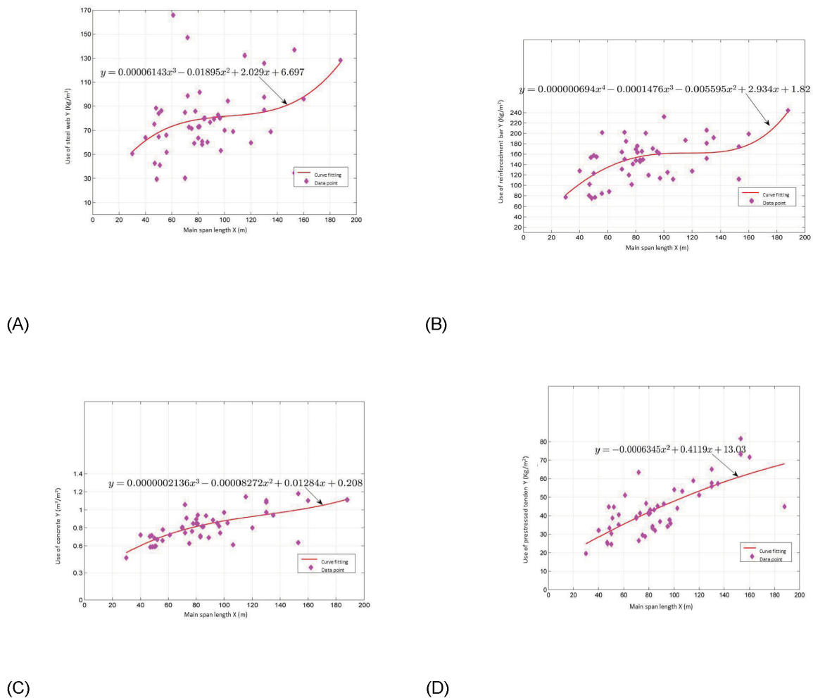
Figure 5. Result of data fitting for material index of girder bridge with corrugated steel web in China and oversea A) Relationship of meter square use of steel web with the main span length; B) Relationship of meter square use of reinforcement bar with the main span length; C) Relationship of meter square use of concrete with the main span length; D) Relationship of meter square use of prestressed tendon with the main span length.
