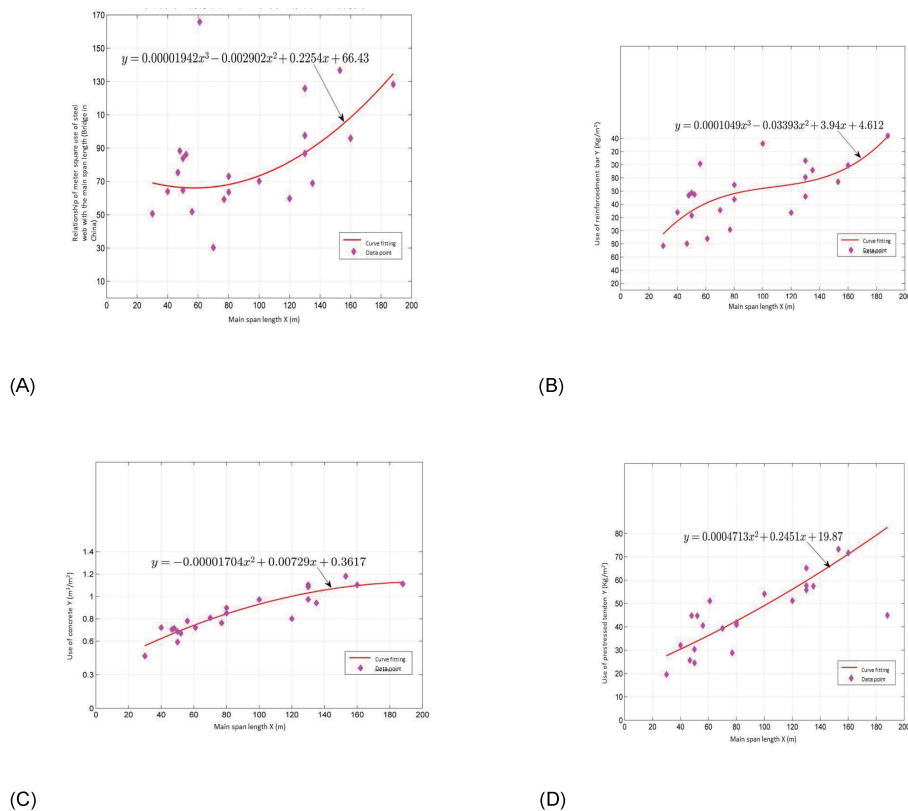
Figure 3. Result of data fitting for material index of girder bridge with corrugated steel web in China. A) Relationship of meter square use of steel web with the main span length; B) Relationship of meter square use of reinforcement bar with the main span length; C) Relationship of meter square use of concrete with the main span length; D) Relationship of meter square use of prestressed tendon with the main span length.
