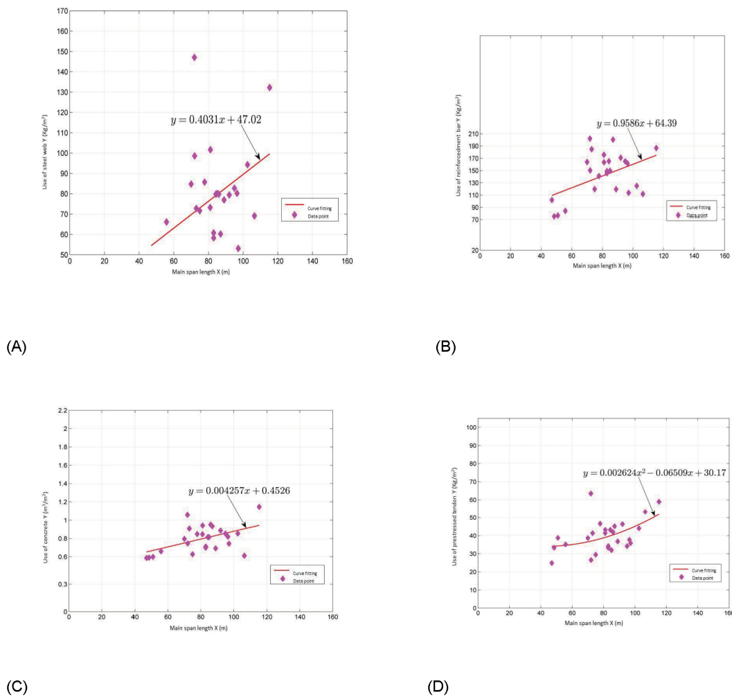
Figure 4. Result of data fitting for material index of overseas girder bridge with corrugated steel web. A) Relationship of meter square use of steel web with the main span length; B) Relationship of meter square use of reinforcement bar with the main span length; C) Relationship of meter square use of concrete with the main span length; D) Relationship of meter square use of prestressed tendon with the main span length.
